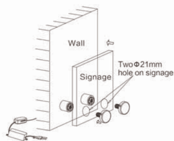
L-2525- 2 (2 sign standoffs +1 power)
